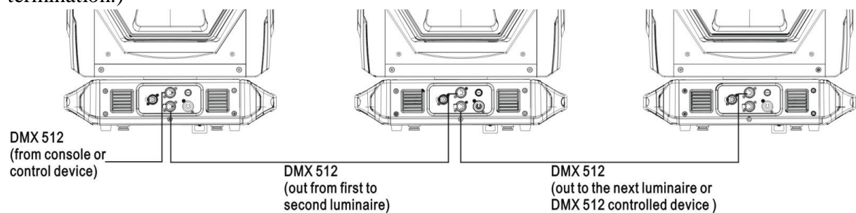
Figure 2-4: Data Link
