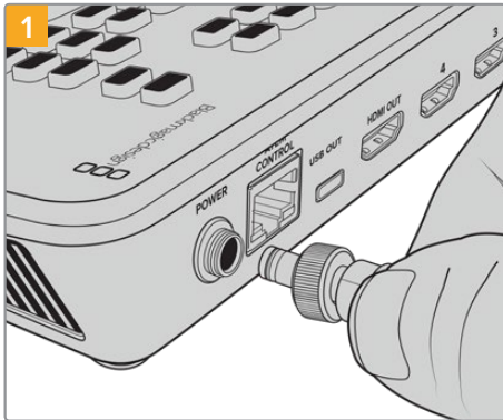
1 Connect power to ATEM Mini's power input using the supplied cable
